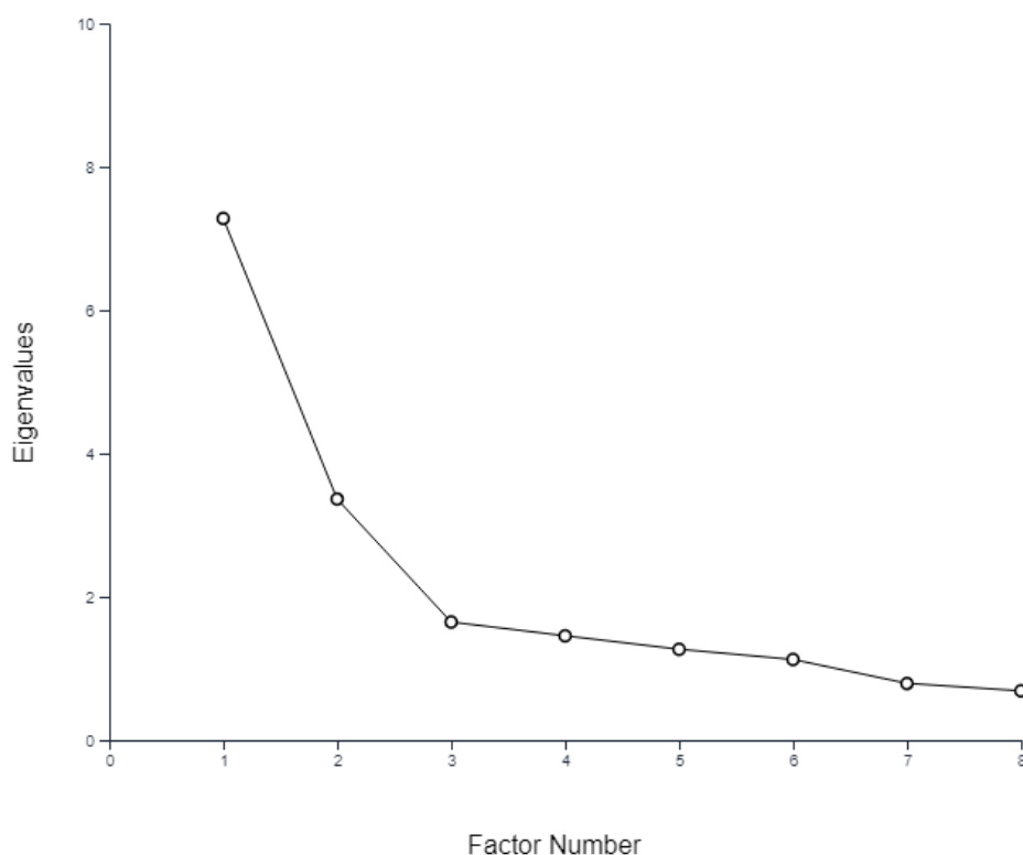
Figure 1. Scree plot chart
